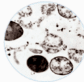
Bacteria after the effect of silver ions
