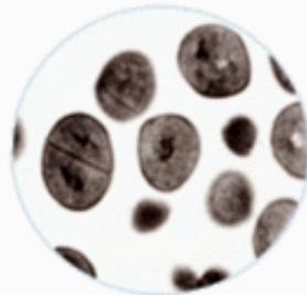
Bacteria before the effect of silver ions
